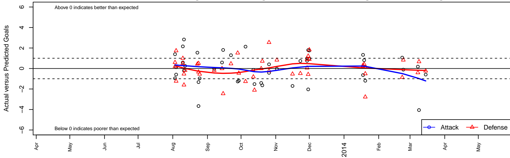
United FC Black B01 Dots are actual minus expected GF (blue circles) and GA (red triangles). Blue line is smoothed change in attack strength. Red is smoothed change in defense strength.
